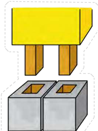
Tenons and sockets
